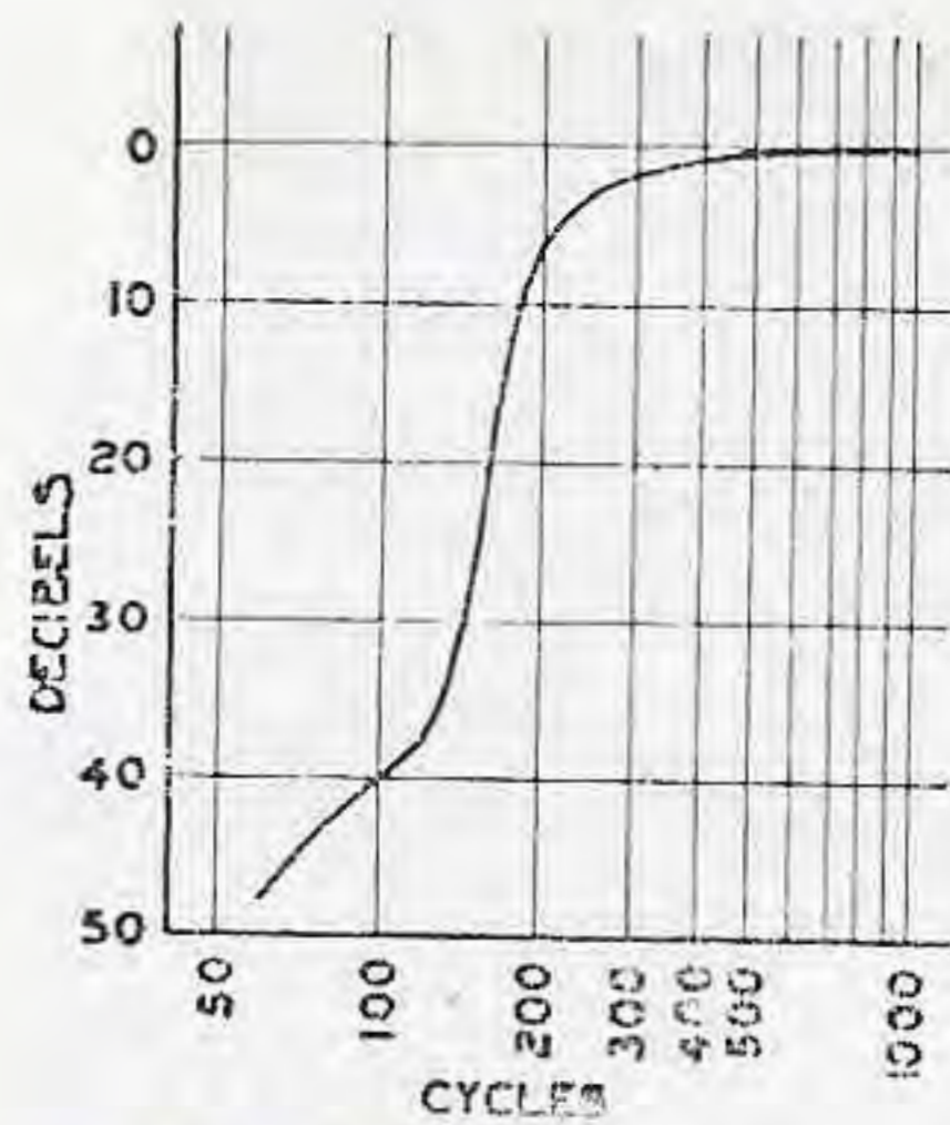
TYPICAL HPI CURVE
