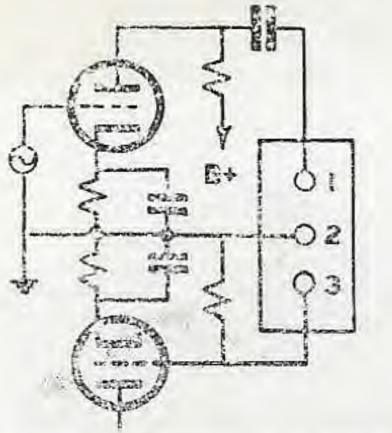
INTERSTAGE FILTER CONNECTIONS
