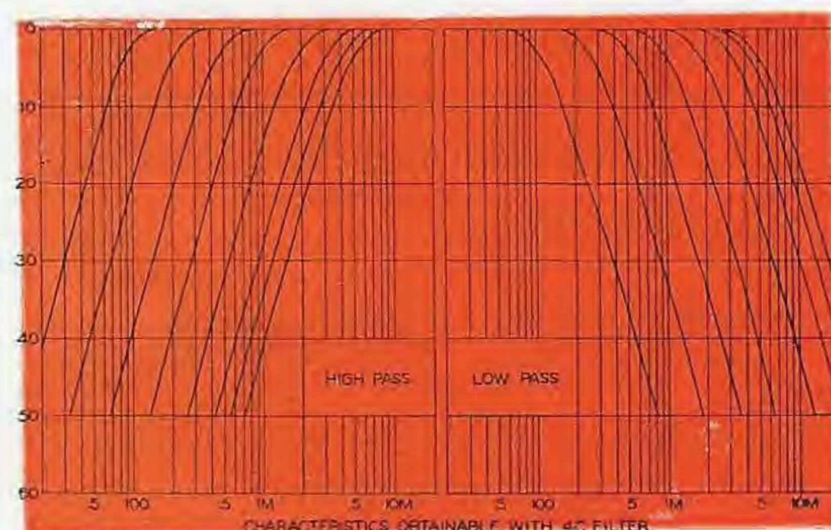
CHARACTERISTICS OBTAINABLE WITH 4C FILTER
